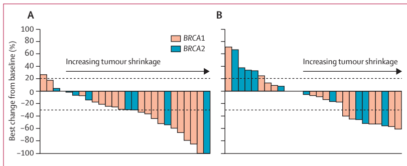
Figure 2: Best percentage change from baseline in target lesion size by BRCA mutation genotype in the intention-to-treat population (A) Olaparib 400 mg twice daily. (B) Olaparib 100 mg twice daily. Reference lines indicate boundaries for progressive disease (20%) and partial response (-30%).
